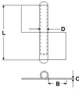
RIGHT HAND HINGE
