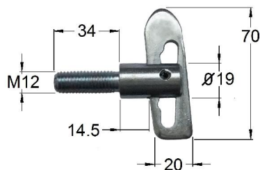
Code no. 98-0705 BOLT-ON DROP LOCK Zinc plated steel
