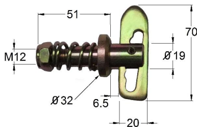
Code no. 98-0745 DROP LOCK Yellow passivated steel
