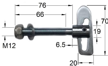
Code no. 98-0703 BOLT-ON DROP LOCK Zinc plated steel
