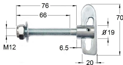
Code no. 98-0706 BOLT-ON DROP LOCK Zinc plated steel
