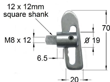
Code no. 98-0713 WELD-ON DROP LOCK Zinc plated
